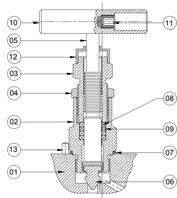
BONNET ASSEMBLY
