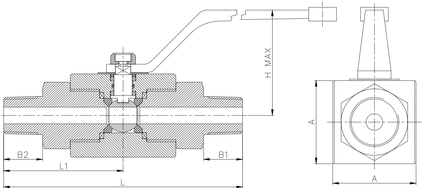
Dimensions (in millimeters)
