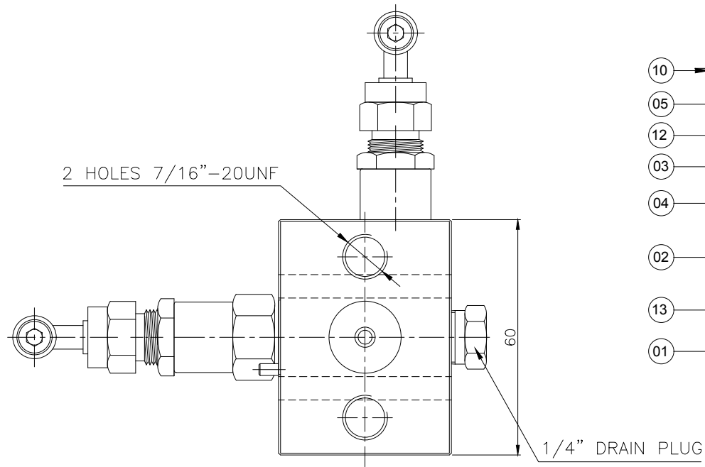
BONNET ASSEMBLY
