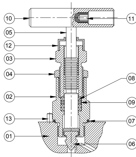
BONNET ASSEMBLY
