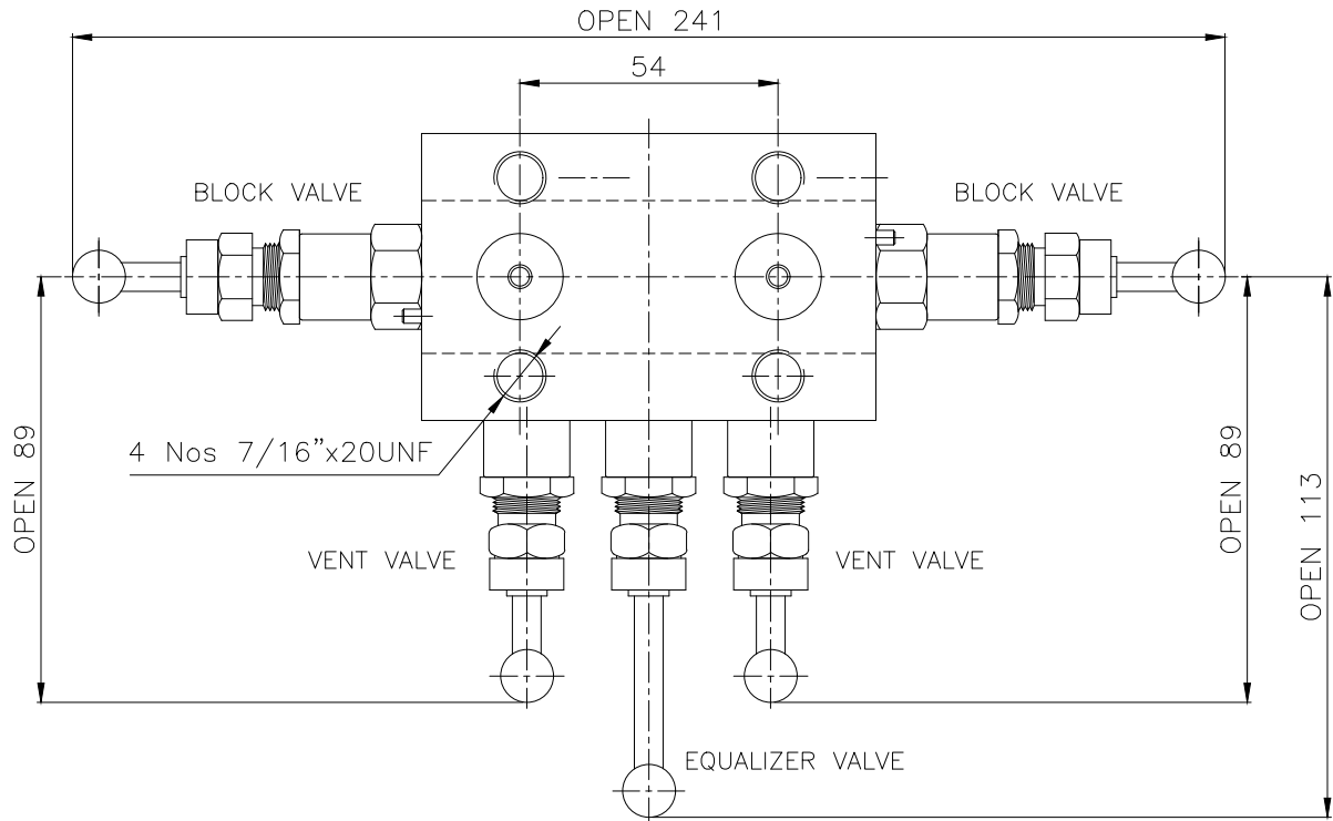
VIEW:- 'AA'
