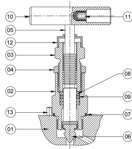
BONNET ASSEMBLY
